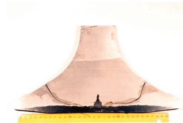
Figure 13: Macro cut through the center of a valve head (RTA62 Nimonic-type 6,430 hrs after repair)
