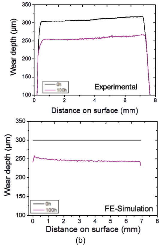
Figure 11. Wear depth profiles from experiment and FE simulation generated wear depths in test mode II on (a) valve spindle (Tribaloy™ T800 material) and (b) seat ring (Tribaloy™ T400 material) at F_N=150 kN, T=450 °C
