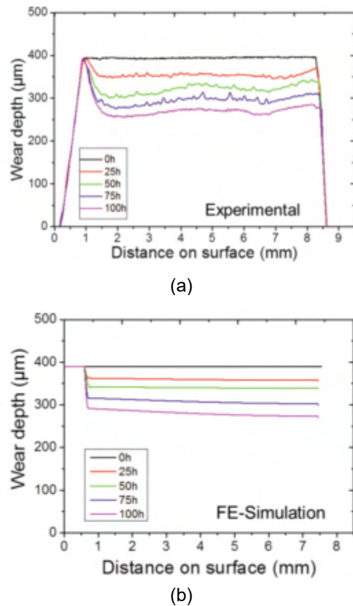
Figure 9. Wear depth profiles on valve spindle (Stellite™ 12 material) in test mode II (a) from experiment and (b) from FE simulation at F_N=80 kN, T=380 °C
