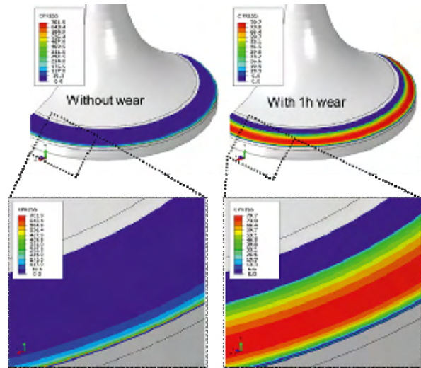
Figure 7. FE-generated contours showing the contact pressure without (left) and with (right) wear after 1 hour at F_N=80 kN, T=330 °C
