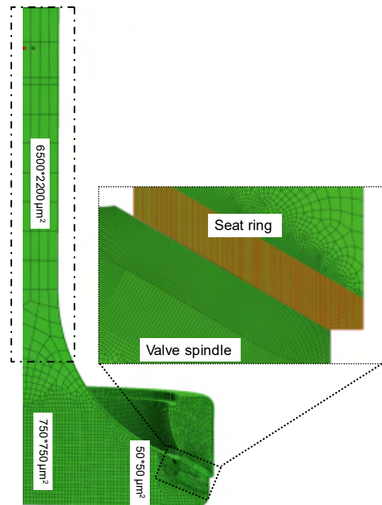
Figure 5. Axisymmetric model with mesh used for finite element simulations
